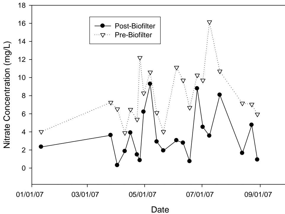
Figure 16. 2007 Conventional drainage bio-filter nitrate data.
