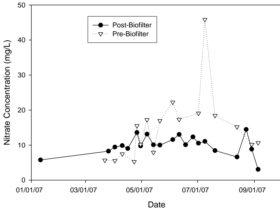
Figure 19. 2007 Shallow drainage bio-filter nitrate data.
