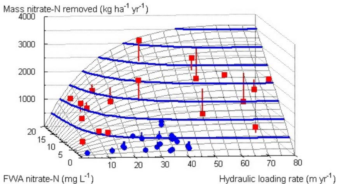
Figure 25. Observed nitrate mass removal includes Corn Belt wetlands representing 46 “wetland years” of data shown (adapted from Crumpton et al. (2006)). 2004 to 2009 CREP wetland sites are shown as red squares. Published results for Ohio and Illinois wetlands shown as blue circles.
