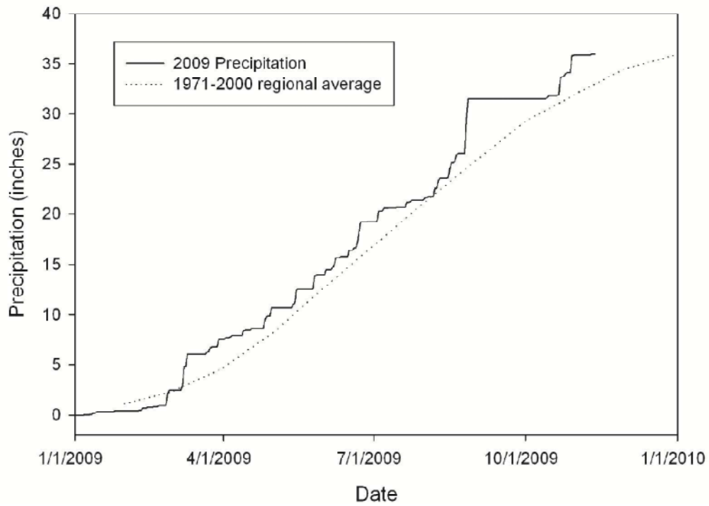
Figure 10. Precipitation in 2009 compared to the 30-year regional average.
