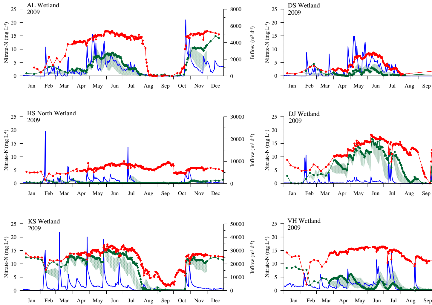
Figure 23. Measured and modeled nitrate concentrations and flows for selected wetlands monitored during 2009.
