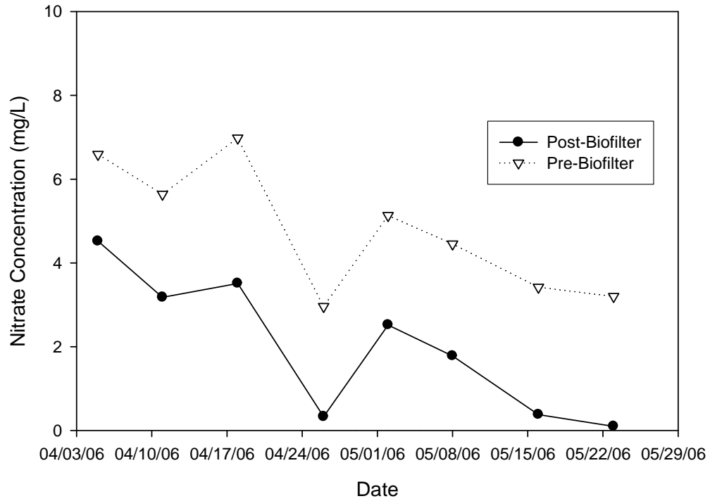
Figure 15. 2006 Conventional drainage bio-filter nitrate data.
