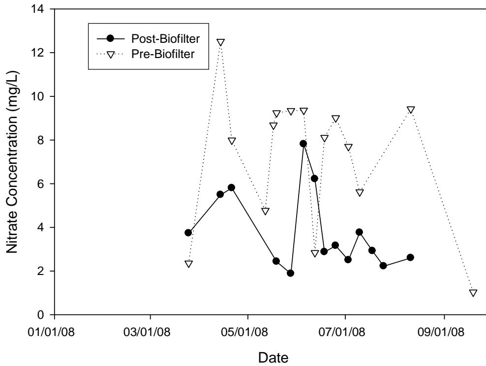
Figure 20. 2008 Shallow drainage bio-filter nitrate data.
