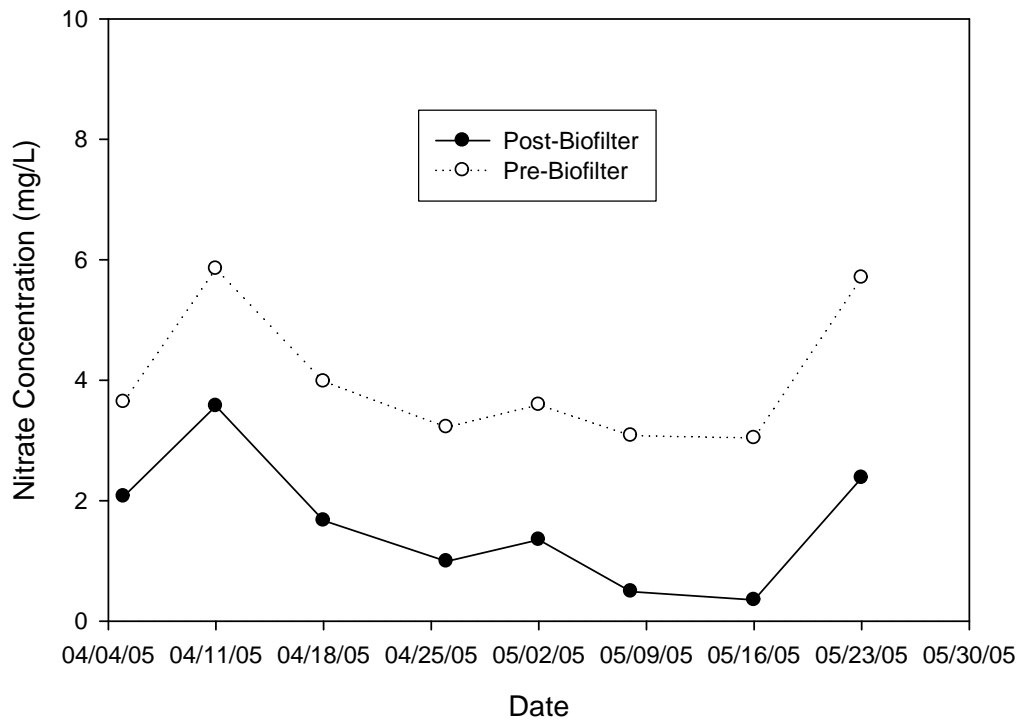
Figure 14. 2005 Conventional drainage bio-filter nitrate data.
