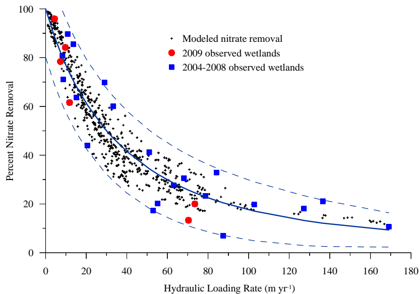
Figure 24. Modeled and observed nitrate removal efficiencies for CREP qualifying wetlands versus Hydraulic Loading Rate based on 1980 to 2005 input conditions.
