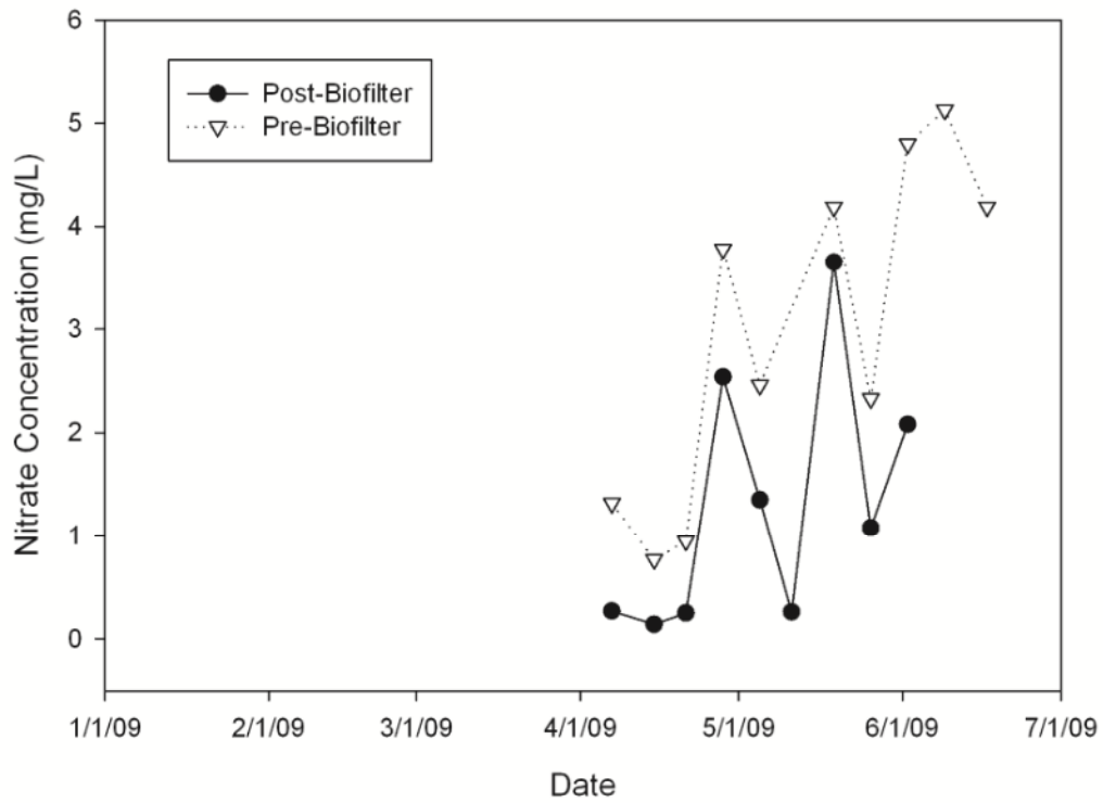
Figure 18. 2009 Conventional drainage bio-filter nitrate data.
