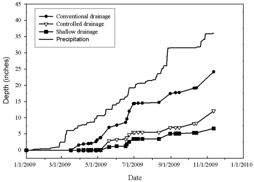
Figure 11. Precipitation and subsurface drainage at the Pekin site in 2009 during the monitoring period.
