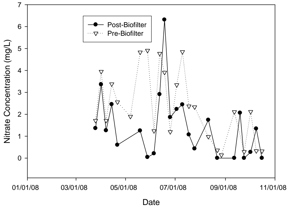
Figure17. 2008 Conventional drainage bio-filter nitrate data.
